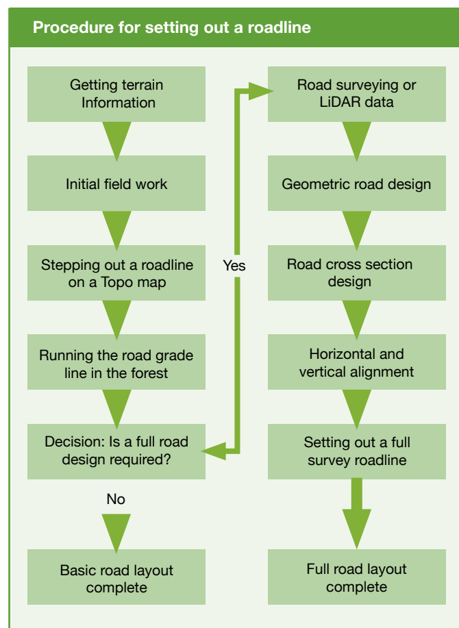
Planning, designing and setting out a roadline
