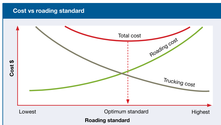
Cost vs road standard. Note that the optimum road standard is a compromise between minimising road construction cost, through-life maintenance cost and trucking cost
