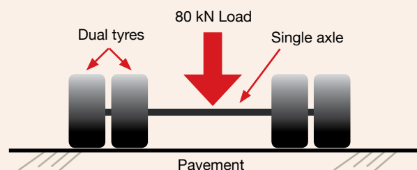
Standard 80 kN axle used for the equivalent standard axle (ESA) load method
