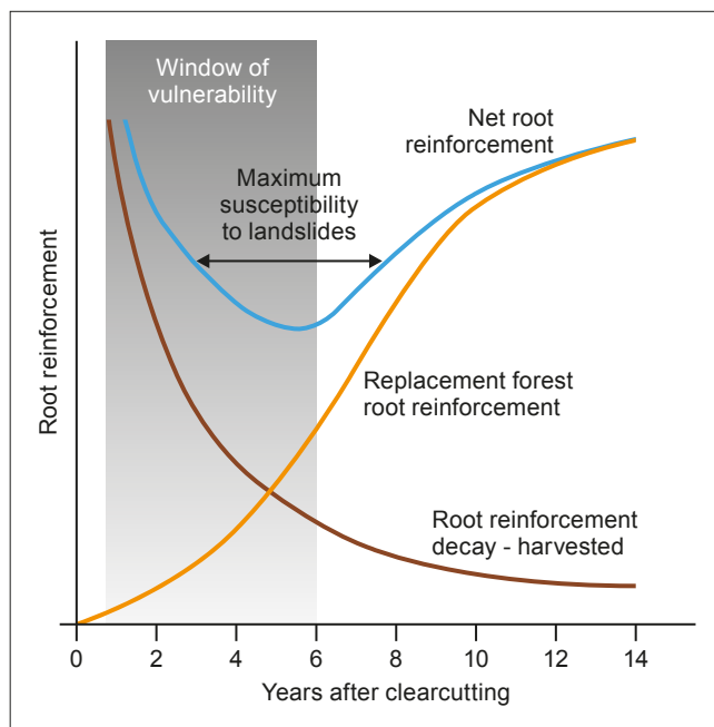
An example of typical changes in forest vegetation root strength or root reinforcement after timber harvesting showing the 'window of vulnerability' (see Phillips et al. 2012 for more details).
