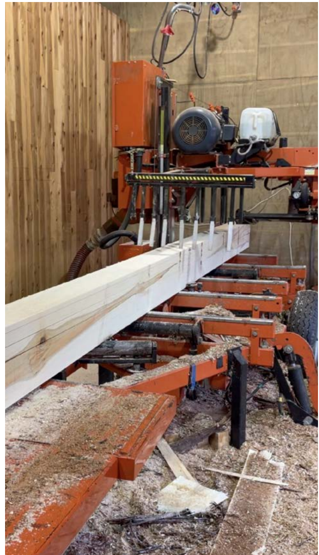
↑ Sawing a poplar log to produce boards for strength testing. Note the pronounced dark heartwood in this clone
