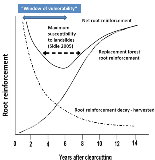
An example of typical changes in forest vegetation root strength or root reinforcement after timber harvesting showing the 'window of vulnerability' (see Phillips et al. 2012 for more details).
